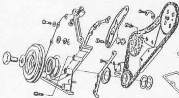
MODEL 99 TIMING CHAIN & COVER
