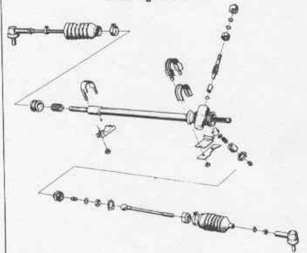
Model 99 Steering Gear
