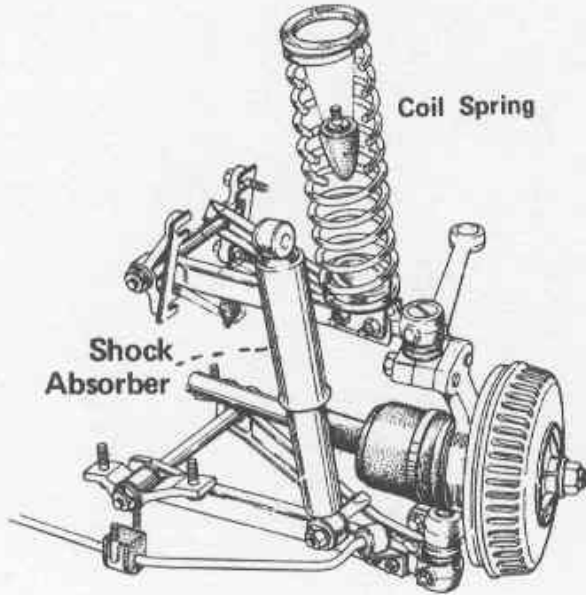
Model 95 & 96 Front Suspension
