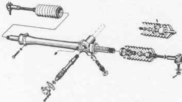
Model 95 & 96 Steering Gear
